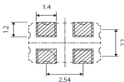
Land Pattern(REFERENCE)
